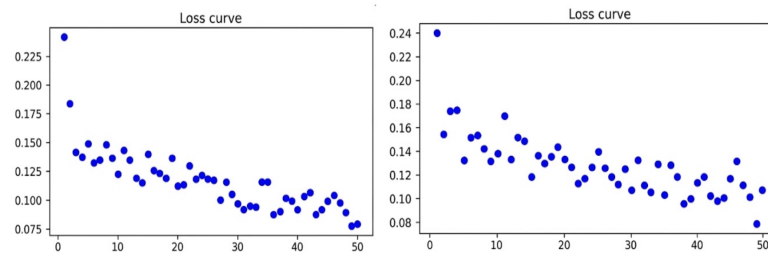
Figure 7. a) Loss curve for real Esrgan pipe lined Nasnet model for Retina dataset b) Loss curve for GFPGAN pipe lined Nasnet model for Retina dataset
