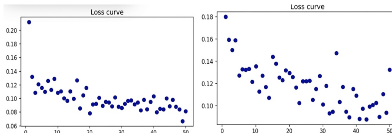
Figure 6. a) Loss curve for real Esrgan pipe lined Nasnet model for Lung dataset b) Loss curve for GFPGAN pipe lined Nasnet t model for lung dataset
