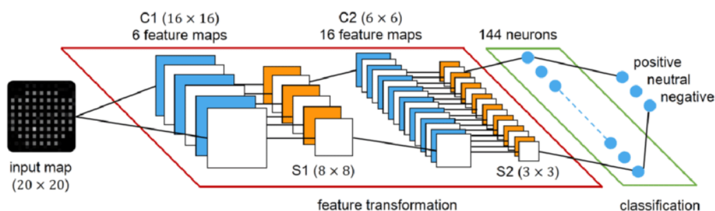
Figure 2. HCNN Network
