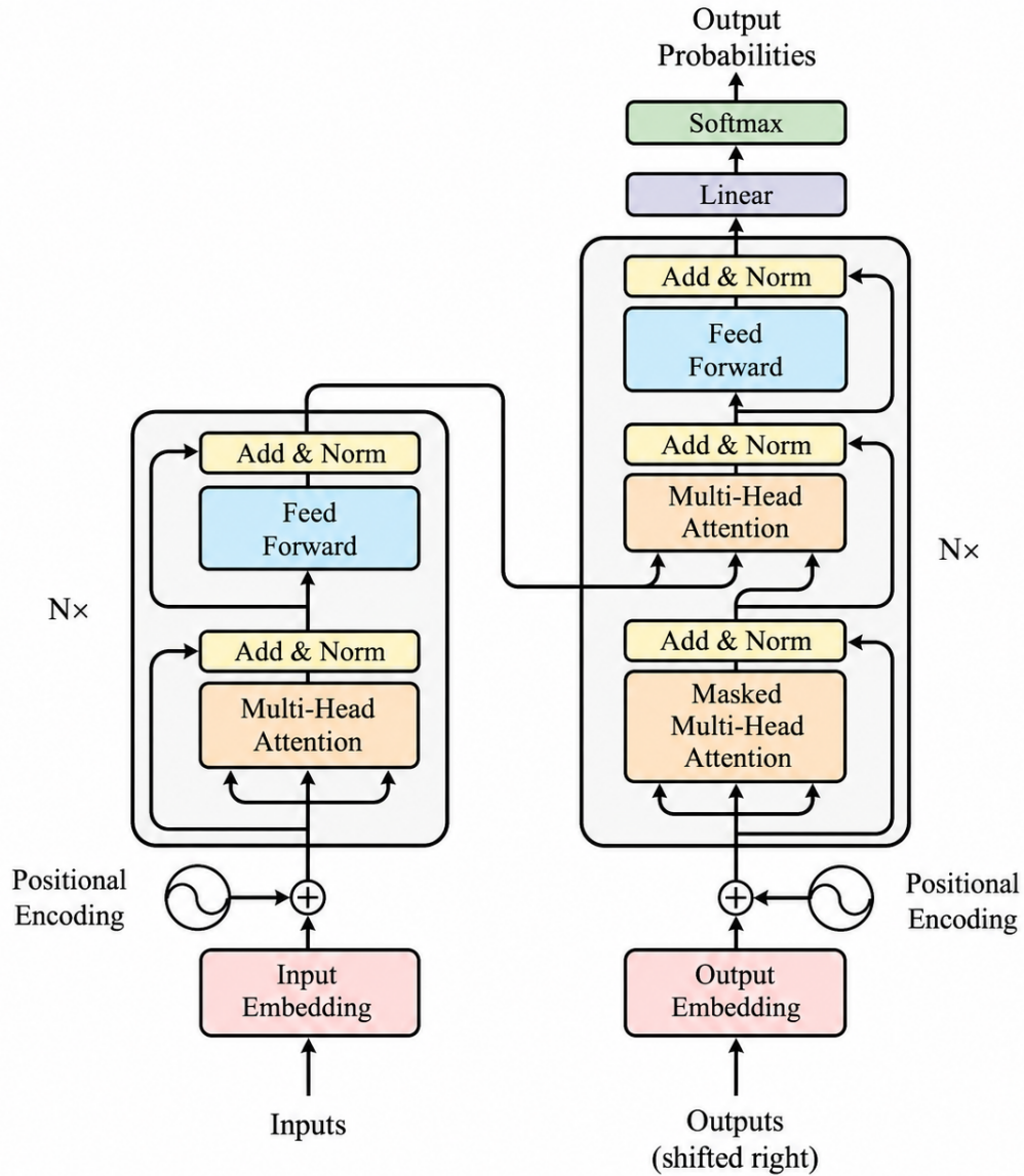
Figure 3. Transformer As Preprocessing Layer
