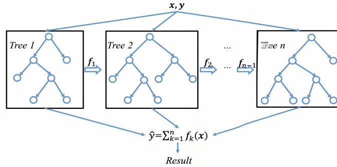
Figure 2. XGBoost Architecture
