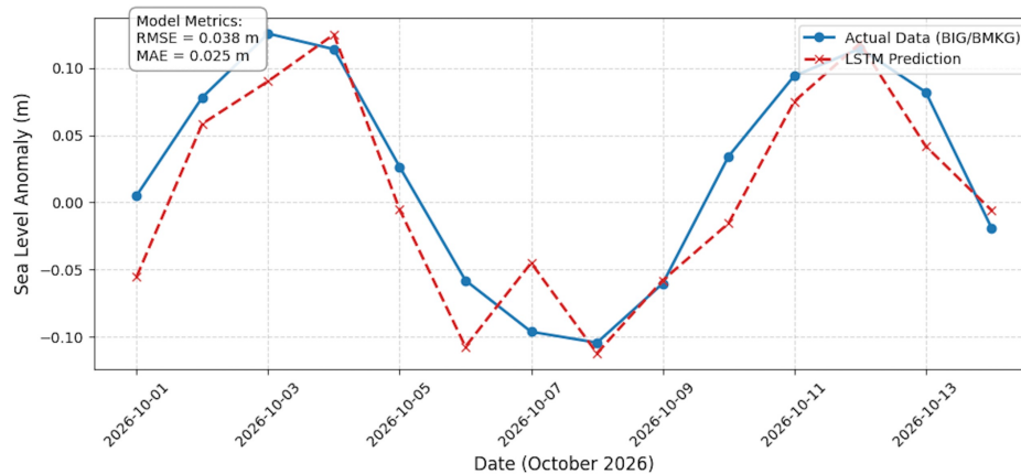
Figure 1. LSTM Model Performance: Observed vs. Predicted Sea-Level Anomalies
